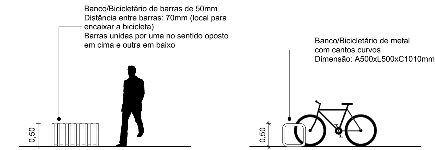
VISTA FRONTAL
